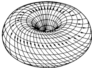
(b) Trajectory eventually covers the surface densely
