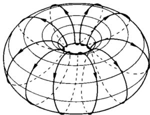
(a) Trajectory closed
